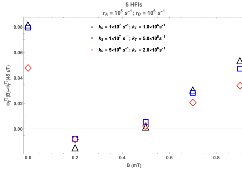
Figure 5: Multiple HFIs: Change in the fractional triplet yield for triplet-born RP with respect to the geomagnetic control (45 \mu T ) as a function of the magnetic field. r_A = 10^5 s^{-1} and r_B = 10^6 s^{-1} . k_S and k_T are singlet and triplet reaction rates, respectively. r_A and r_B are the spin relaxation rates of radicals A and B, respectively. 5 HFIs: H5 ( -802.9 \mu T ), N5 ( 431.3 \mu T ), three H8 ( 255.4 \mu T ) [30].
