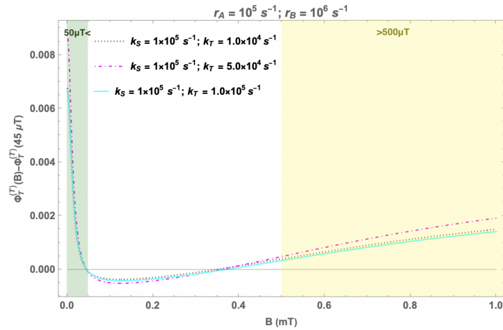
Figure 3: Predictions of the RPM model: Change in the fractional triplet yield for triplet-born flavin-superoxide RP with respect to the geomagnetic control (45 \mu T ) as a function of the magnetic field (0 – 1 mT). r_A = 10^5 s^{-1} and r_B = 10^6 s^{-1} . k_S and k_T are singlet and triplet reaction rates, respectively. r_A and r_B are the spin relaxation rates of radicals A and B, respectively. Again, only the largest isotropic HF coupling (H5) is taken into account (HFCC value is -802.9 \mu T ). The region with sub-geomagnetic fields is shaded in green, and the region with fields greater than 500 \mu T is shaded in yellow.
