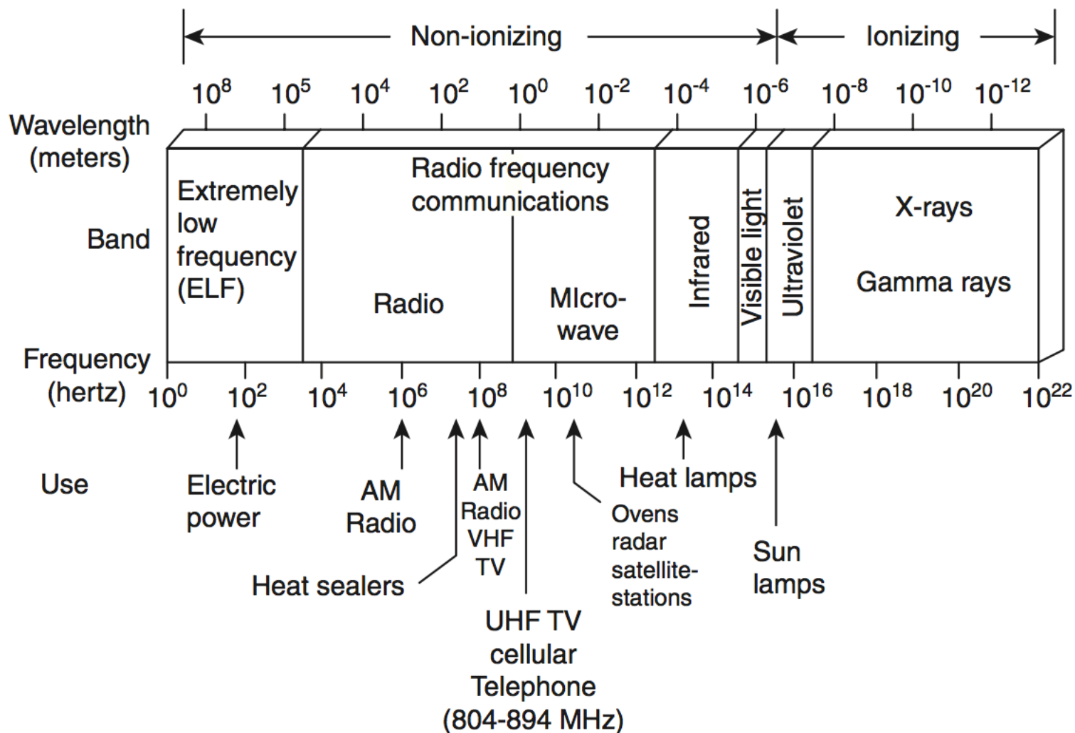
Figure 1 The electromagnetic spectrum.
