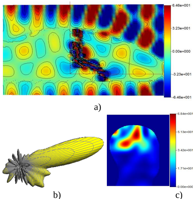
Figure 5. Near field distribution in the car (a) and far field pattern (b), SAR distribution inside of human head (c) at 450 MHz (source is base station antenna).
