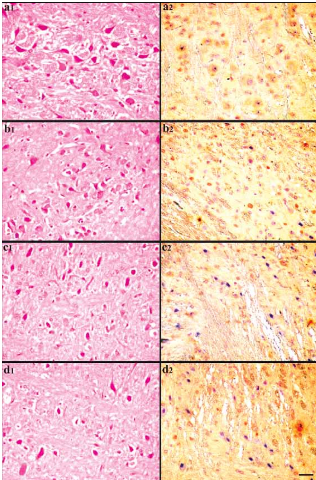
Figure 2: Representative light microphotographs showing the morphology (a1–d1) and apoptosis (a2–d2) of the brain stem tissue in control and EMR groups (900, 1800, 2450 MHz) by hematoxylin-eosin and caspase-3 immunohistochemistry. (Immunoperoxidase, haematoxylin counterstain, scale bar, 50 \mu m) 1 2 3 4 5 6 7 8 9 10 11 12 13 14 15 16.
