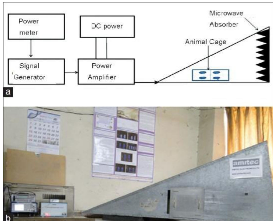
(a) Schematic diagram of microwave exposure setup (b) Photograph of gigahertz transversal electromagnetic cell
