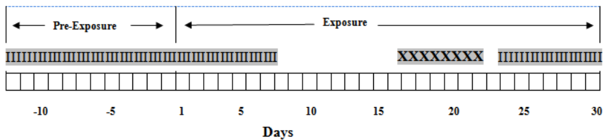
Figure 1. Diagrammatic representation of the period of monitoring of wheel running activity (IIII) and Water maze test (XXXX) with reference to exposure to microwave radiation.
