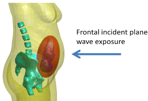
Figure 5. Direction of arrival of the incident plane wave.
