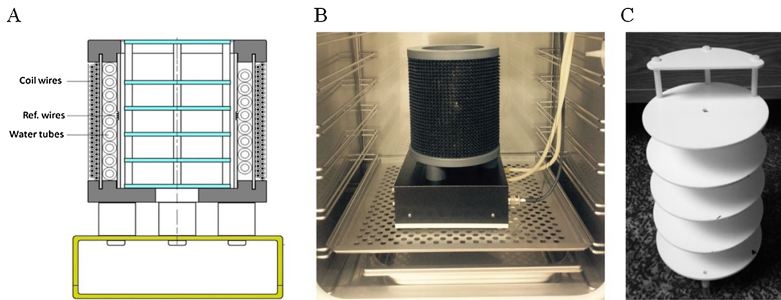
Fig. 2. The IF exposure system. A: scheme of the solenoid IF exposure system. B: the solenoid coil exposure system placed in the CO 2 incubator. C: Sample holder within the solenoid coil.
