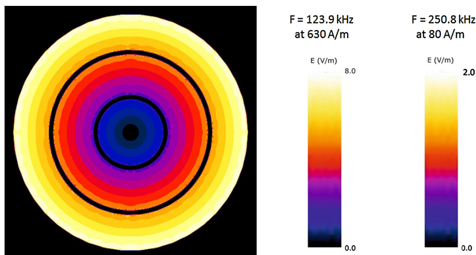
Fig. 4. Distribution of induced electric field (V/m) within the sample of each separated annular ring at 123.9 kHz and 250.8 kHz frequencies under exposure to 630 A/m and 80 A/m magnetic field, respectively. The maximum induced electric field (E) in samples were 7.97 V/m at 123.9 kHz and 2.04 V/m at 250.8 kHz at the edge of outer ring, respectively. F represents frequency in kHz.
