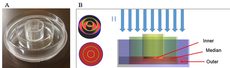
Fig. 3. A: Petri dish system divided cylindrically into three parts by concentric rings. B: Simulated uniform magnetic field (H) perpendicular to Petri dish with blood sample.
