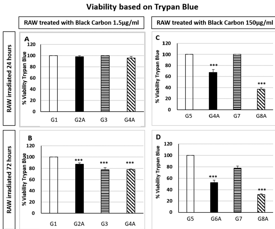
Fig. 1. Histograms showing the percentage of cell viability using Trypan blue: (A) group treated with BC 1.5 µg/ml and irradiated during 24 h; (B) group treated with BC 1.5 µg/ml and irradiated during 72 h; (C) group treated with BC 150 µg/ml and irradiated during 24 h; (D) group treated with BC 150 µg/ml and irradiated during 72 h. In G1 (RAW non-radiated 24 h), G2A (RAW BC 1.5 µg/ml + no RAD 24 h), G2B (RAW BC 150 µg/ml + no RAD 24 h), G3 (RAW RAD 24 h), G4A (RAW BC 1.5 µg/ml + RAD 24 h), G4B (RAW BC 150 µg/ml + RAD 24 h), G5 (RAW non-radiated 72 h), G6A (RAW BC 1.5 µg/ml + no RAD 72 h), G6B (RAW BC 150 µg/ml + no RAD 72 h), G7 (RAW RAD 72 h), G8A (RAW BC 1.5 µg/ml + RAD 72 h), G8B (RAW BC 150 µg/ml + RAD 72 h) groups. *** Indicates significant differences in relation to the non-radiated group ( p < 0.001 ). Ninety-six samples were used, six for each group/time. Mean values are shown (six samples for each group/time). Error bars indicate the standard error of mean (SEM) within each group (radiated with/without BC, only BC or non-radiated). (For interpretation of the references to colour in this figure legend, the reader is referred to the web version of this article.)
