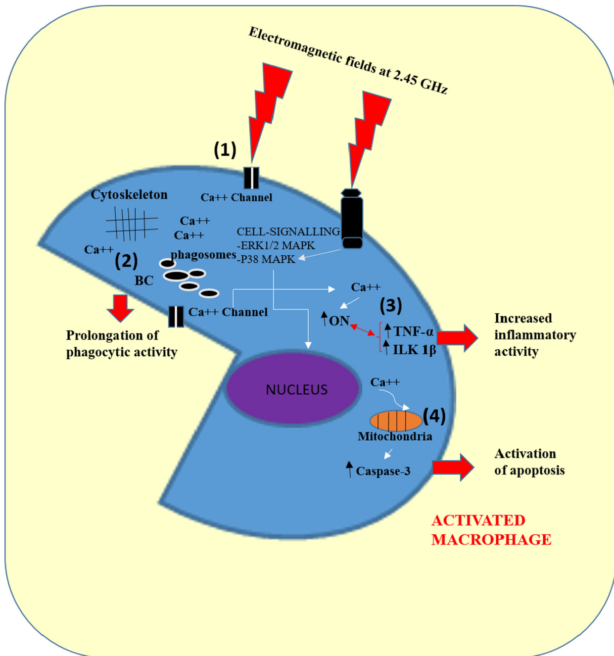
Fig. 6. Illustrations explaining the hypothesis of the mechanism by which RF at 2.45 GHz and the Black Carbon (BC) in the activated macrophage would act in combination. (1) RF and BC stimulate the ion channels [Ca 2+ ] and facilitate the entry of the ion at the intracytoplasmic level (2), causing alteration of the cytoskeleton and prolongation of phagocytic activity (3) along with increased inflammatory activity and release of NO, TNF-α and interleukin 1β, (4) which activates the apoptosis cascade by increasing caspase-3.
