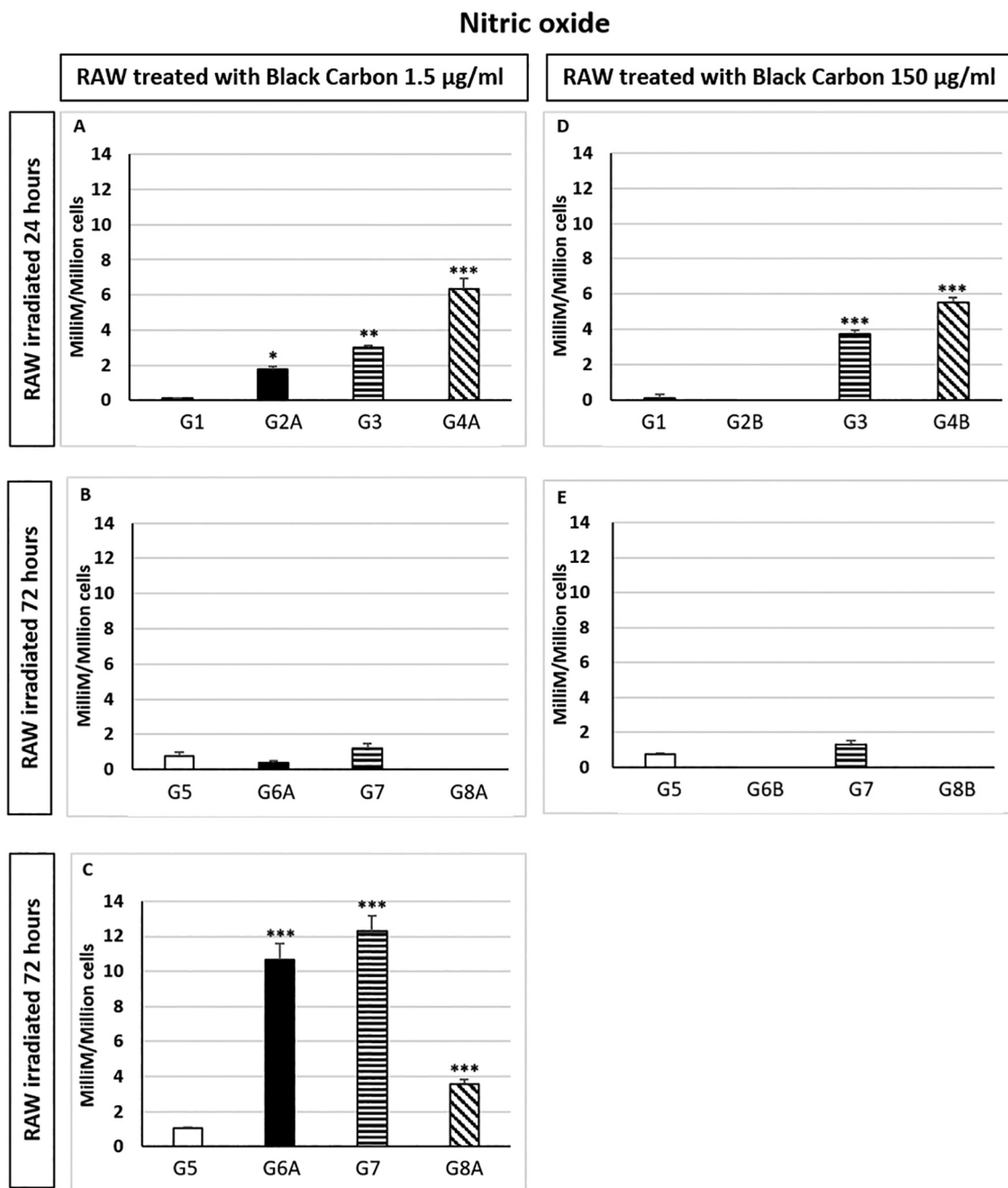
Fig. 3. Histograms showing nitric oxide concentration: (2A) nitric oxide concentrations at 24 h after RAW treatment with BC 1.5 \mu\text{g/ml} and irradiated during 24 h; (2B) nitric oxide concentrations at 24 h after RAW treatment with BC 1.5 \mu\text{g/ml} and irradiated during 72 h; (2C) nitric oxide concentrations at 72 h after RAW treatment with BC 1.5 \mu\text{g/ml} and irradiated during 72 h. (2D) Nitric oxide concentrations at 24 h after RAW treatment with BC 150 \mu\text{g/ml} and irradiated during 24 h; (2E) nitric oxide concentrations at 24 h after RAW treatment with BC 150 \mu\text{g/ml} and irradiated during 72 h in G1 (RAW non-irradiated 24 h), G2A (RAW BC 1.5 \mu\text{g/ml} + no RAD 24 h), G2B (RAW BC 150 \mu\text{g/ml} + no RAD 24 h), G3 (RAW RAD 24 h), G4A (RAW BC 1.5 \mu\text{g/ml} + RAD 24 h), G4B (RAW BC 150 \mu\text{g/ml} + RAD 24 h), G5 (RAW non-irradiated 72 h), G6A (RAW BC 1.5 \mu\text{g/ml} + no RAD 72 h), G6B (RAW BC 150 \mu\text{g/ml} + no RAD 72 h), G7 (RAW RAD 72 h), G8A (RAW BC 1.5 \mu\text{g/ml} + RAD 72 h), G8B (RAW BC 150 \mu\text{g/ml} + RAD 72 h) groups. Values were transformed based on percentage of viability for each group. Mean values are shown (six samples for each group/time). Error bars indicate the standard error of mean (SEM) within each group (irradiated with/without BC, only BC or non-irradiated). Significant differences in relation to the non-treated group are also shown: * ( p < 0.05 ); ** ( p < 0.01 ); *** ( p < 0.001 ).
