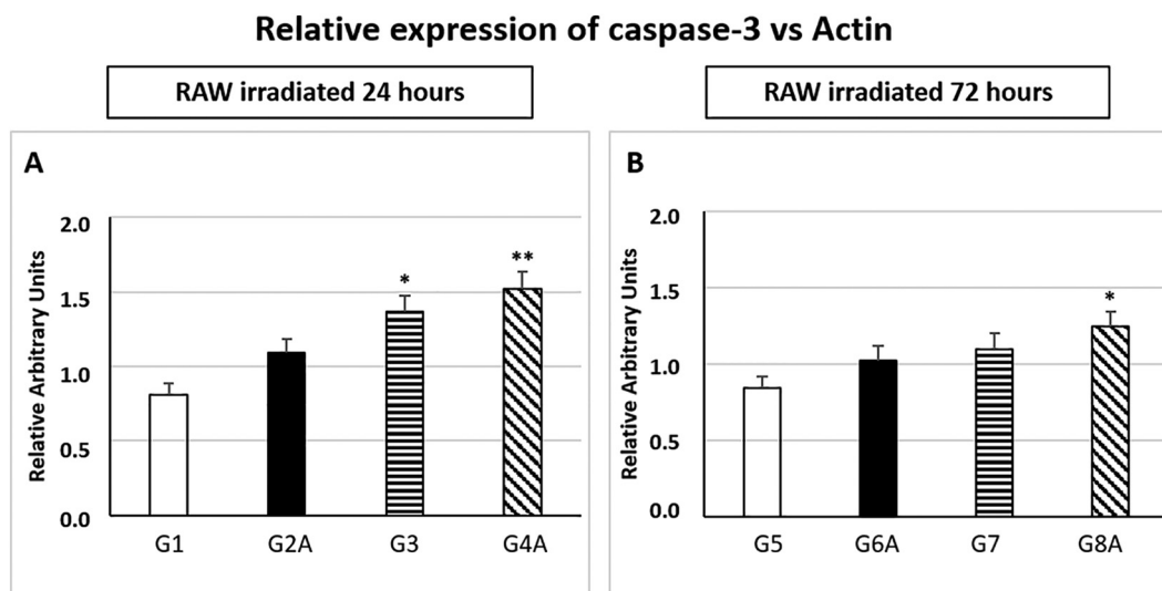
Fig. 5. Histograms of mRNA expression of caspase-3 protein (5A) RAW treated 24 h. (5B) RAW treated 72 h in G1 (RAW non-irradiated 24 h), G2A (RAW BC 1.5 \mu\text{g/ml} + no RAD 24 h), G3 (RAW RAD 24 h), G4A (RAW BC 1.5 \mu\text{g/ml} + RAD 24 h), G5 (RAW non-irradiated 72 h), G6A (RAW BC 1.5 \mu\text{g/ml} + no RAD 72 h), G7 (RAW RAD 72 h), G8A (RAW BC 1.5 \mu\text{g/ml} + RAD 72 h) groups. Mean values are shown (six samples for each group/time). Error bars indicate the standard error of mean (SEM) within each group (irradiated with/without BC, only BC or non-irradiated). Significant differences in relation to the non-treated group are also shown: * ( p < 0.05 ); ** ( p < 0.01 ).
