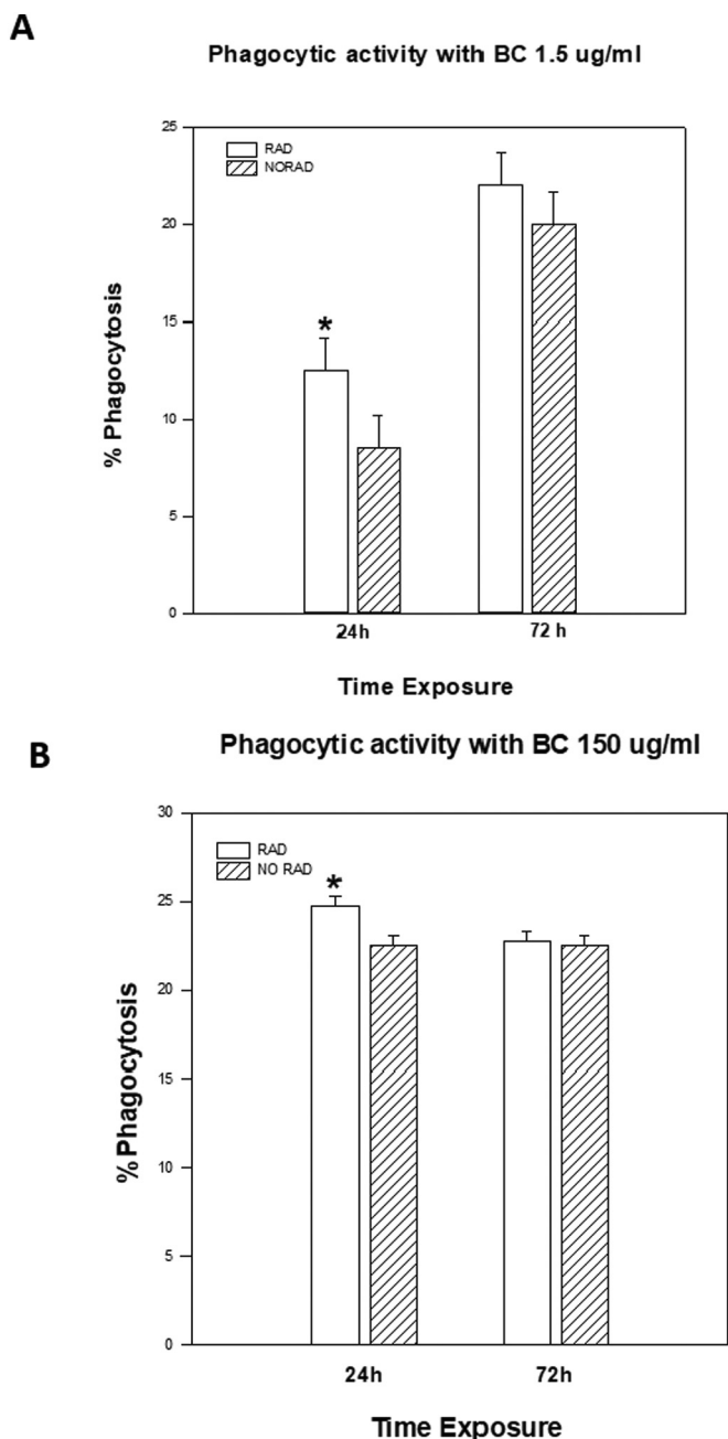
Fig. 2. Histograms showing the evolution of the phagocytosis rate (%) in 24/72 h: (A) phagocytic activity with BC 1.5 \mu\text{g}/\text{ml} ; (B) phagocytic activity with BC 150 \mu\text{g}/\text{ml} . In (A) G2A (RAW BC 1.5 \mu\text{g}/\text{ml} + no RAD 24 h), G4A (RAW BC 1.5 \mu\text{g}/\text{ml} + RAD 24 h), G6A (RAW BC 1.5 \mu\text{g}/\text{ml} + no RAD 72 h), G8A (RAW BC 1.5 \mu\text{g}/\text{ml} + RAD 72 h) in (B) G2B (RAW BC 150 \mu\text{g}/\text{ml} + no RAD 24 h), G4B (RAW BC 150 \mu\text{g}/\text{ml} + RAD 24 h), G6B (RAW BC 150 \mu\text{g}/\text{ml} + no RAD 72 h), G8B (RAW BC 150 \mu\text{g}/\text{ml} + RAD 72 h) groups. * Indicates significant differences in relation to the non-radiated group ( p < 0.001 ). Ninety-six samples were used, six for each group/time. Mean values are shown (six samples for each group/time). Error bars indicate the standard error of mean (SEM) within each group (radiated with/without BC, only BC or non-radiated); (C) microphotographs showing phagocytosis of BC particles in the macrophages, RAW BC 1.5 \mu\text{g}/\text{ml} + RAD 24 h (a) RAW BC 1.5 \mu\text{g}/\text{ml} + RAD 72 h (b) RAW BC 150 \mu\text{g}/\text{ml} + RAD 24 h (c) RAW BC 150 \mu\text{g}/\text{ml} + RAD 72 h (d). Photographs taken at 100 \times magnification. Calibration bar 10 \mu\text{m} .
