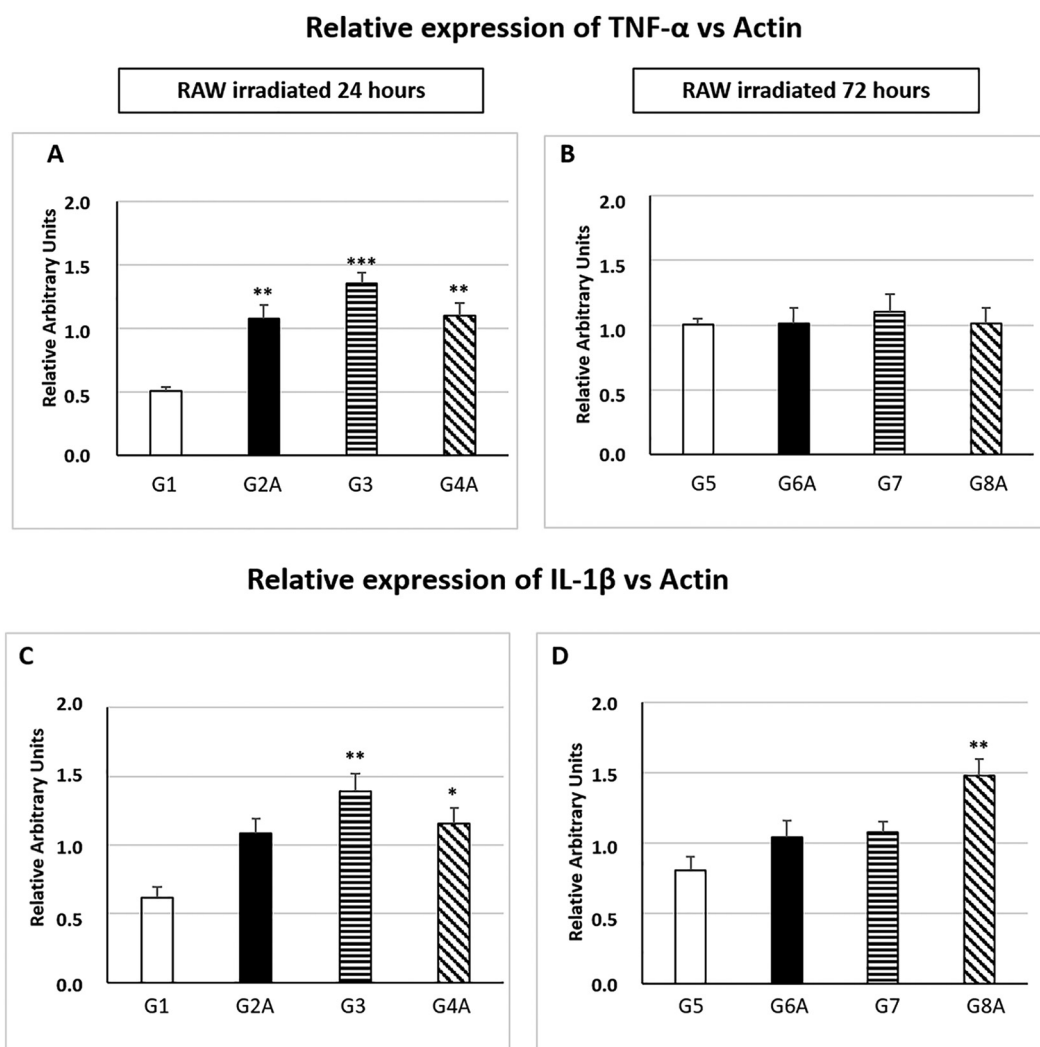
Fig. 4. Histograms of mRNA expression of TNF-α (A and B) and IL-1β (C and D) protein. (4A; 4C) RAW treated 24 h. (4B; 4D) RAW treated 72 h in G1 (RAW non-radiated 24 h), G2A (RAW BC 1.5 µg/ml + no RAD 24 h), G3 (RAW RAD 24 h), G4A (RAW BC 1.5 µg/ml + RAD 24 h), G5 (RAW non-radiated 72 h), G6A (RAW BC 1.5 µg/ml + no RAD 72 h), G7 (RAW RAD 72 h), G8A (RAW BC 1.5 µg/ml + RAD 72 h) groups. Mean values are shown (six samples for each group/time). Error bars indicate the standard error of mean (SEM) within each group (radiated with/without BC, only BC or non-radiated). Significant differences in relation to the non-treated group are also shown: * ( p < 0.05 ); ** ( p < 0.01 ); *** ( p < 0.001 ).
