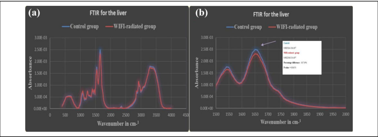
Figure 2. (a) Average FTIR spectra from rat liver tissue. Blue: control group; red: Wi-Fi-radiated group. (b) Zoom of the wavenumber part from 1500 cm −1 to 2000 cm −1 of the FTIR spectrum. FTIR: Fourier transform infrared.
