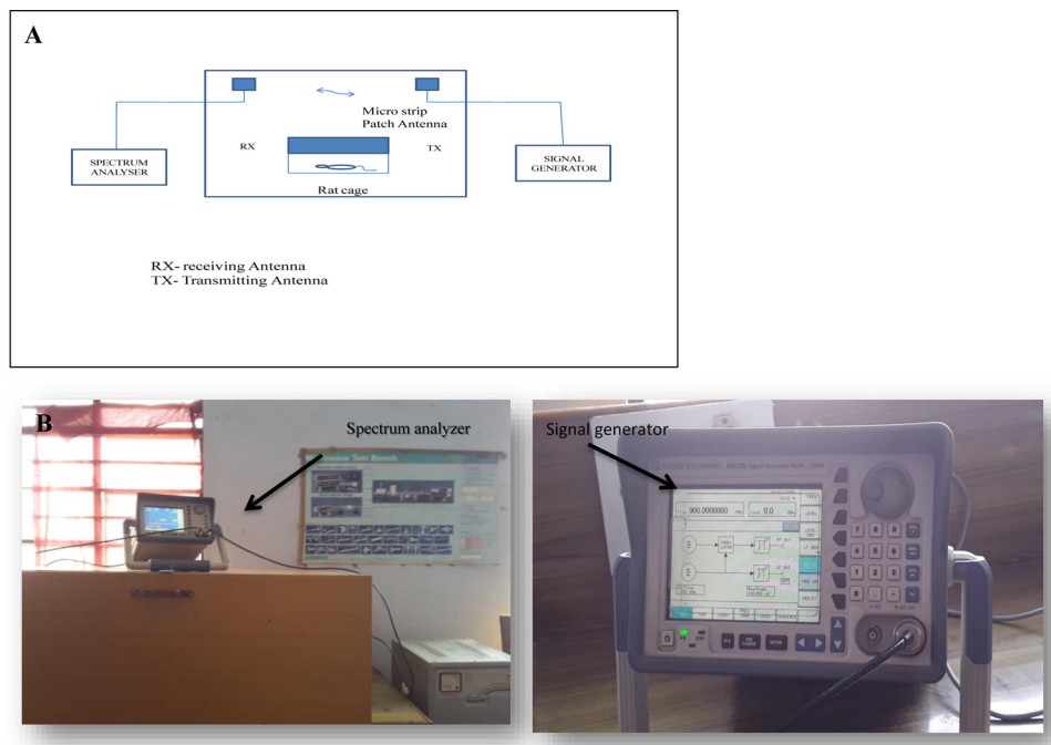
Fig. 1. A-B. Demonstrated the layout and schematic design of exposure setup.
