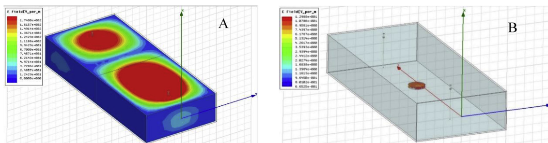
Fig. 1. Simulation of the electromagnetic field using the HFSS software. A) A screenshot of a progressive electromagnetic field inside the cavity. The red and blue zones are corresponded to the maximum and minimum homogeneity of electromagnetic field, respectively. B) A Cross-section of the electric field on the cell samples determined via HFSS simulation. (For interpretation of the references to colour in this figure legend, the reader is referred to the Web version of this article.)
