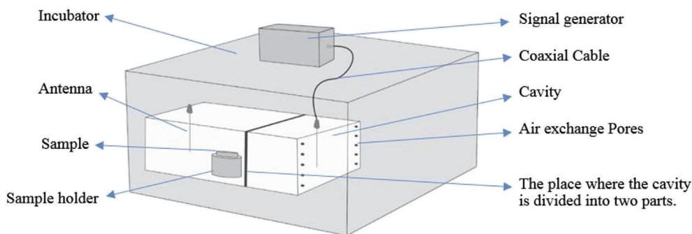
Fig. 2. A graphic picture of RFR-exposure set-up.
