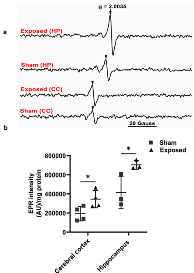
Fig. 2. Exposure to radiofrequency electromagnetic radiation (RF-EMR) for 8 h increased the level of carbon centered free radicals in the developing rat brain. a. Representative images of electron paramagnetic resonance (EPR) spectra showing a clear peak of g = 2.0035 radical species in the cerebral cortex (CC) and hippocampus (HP) region of sham and RF-EMR-exposed rats. b. A Scatter dot plot is showing a statistical comparison of EPR signal intensity between groups ( n = 4 ). EPR signal intensity was obtained by measuring peak to peak height of the central signal which is an estimate of radical concentration and expressed in arbitrary units (a.u.)/mg protein. Data presented as mean \pm standard error of the mean (SEM). Two-tailed unpaired t-test. * P \leq 0.05 , significantly different from the sham group.
