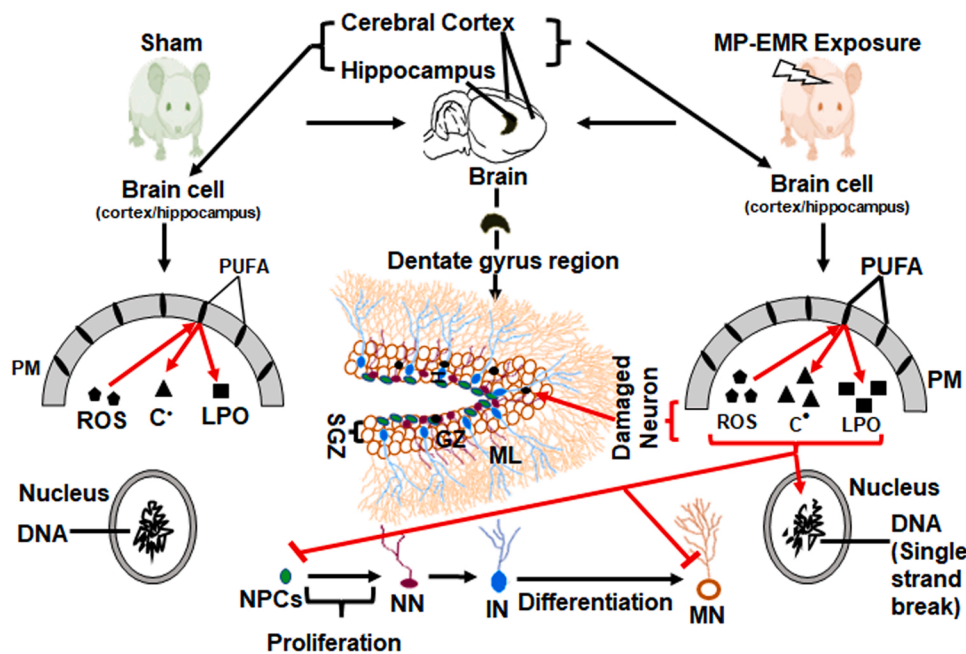
Fig. 9. Exposure to radiofrequency electromagnetic radiation (RF-EMR) seems to induce reactive oxygen species (ROS) production, which targets polyunsaturated fatty acids (PUFA) in the cerebral cortex and hippocampus cell membrane and generates carbon-centered radicals (C•) and lipid peroxides (LPO) leading to DNA damage, neuronal degeneration and impaired proliferation of hippocampal neural progenitor cells (NPCs). Important outcomes and their possible role and interrelationship at the cellular level are presented. BrdU: 5-Bromo-2'-deoxyuridine, GZ: granular zone, H: hilus, IN: immature neurons, ML: molecular layer, MN: mature neurons, NN: newborn neurons, PM: plasma membrane, RF: radiofrequency, SGZ: sub-granular zone.
