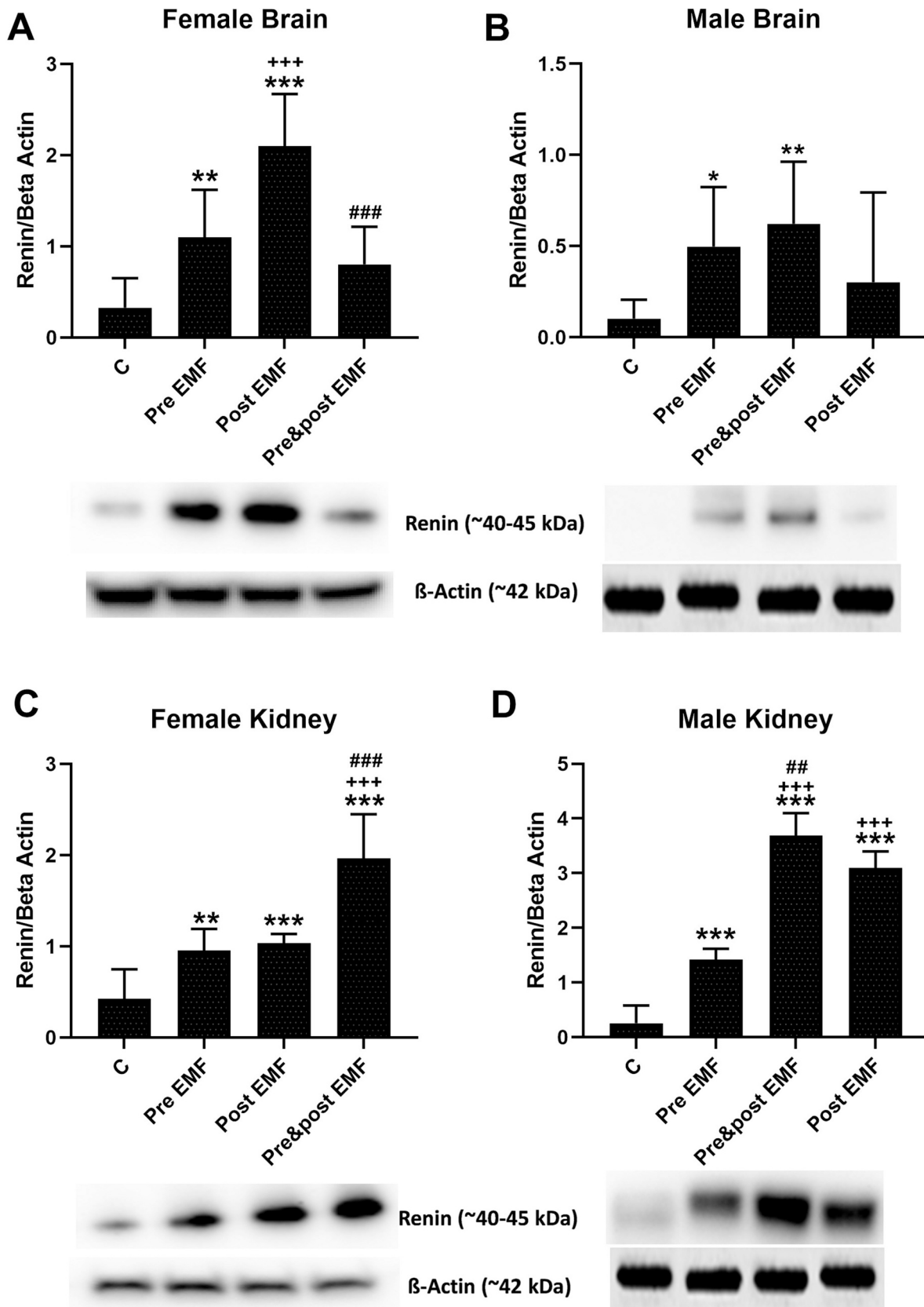
Fig. 3. Western blotting assay results of renin for female brain tissue (n = 9) (A), male brain tissue (n = 9) (B), female kidney tissue (n = 9) (C) and male kidney tissue (n = 9) (D). Data were presented as mean ± SD. *p < 0.05, **p < 0.01, ***p < 0.001 statistical significance compared to C group. +++p < 0.001 compared to the Pre EMF group. ##p < 0.01, ###p < 0.001 compared to the Post EMF group.
