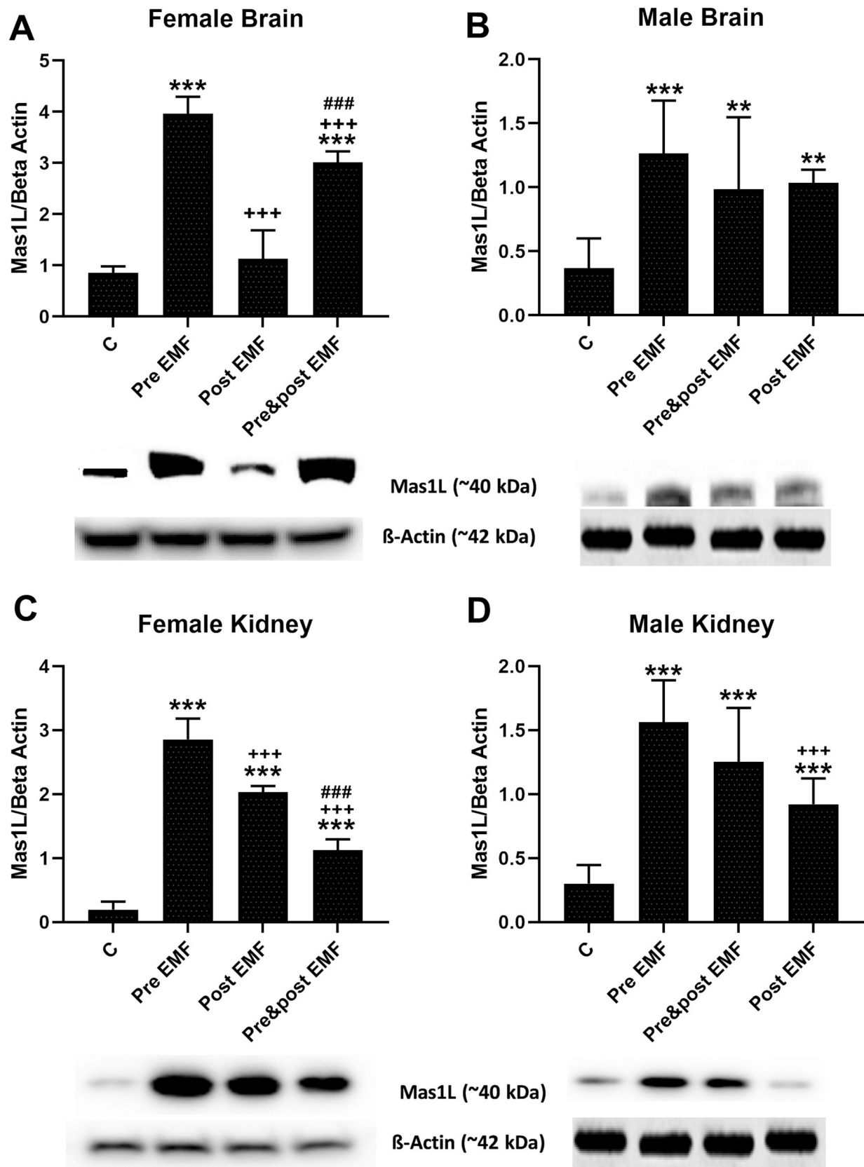
Fig. 7. Western blotting assay results of Mas1L for female brain tissue (n = 9) (A), male brain tissue (n = 9) (B), female kidney tissue (n = 9) (C) and male kidney tissue (n = 9) (D). Mas1L; Mas-related G-protein coupled receptor. Data were presented as mean ± SD. **P < 0.01, ***P < 0.001 statistical significance compared to C group. +++p < 0.001 compared to the Pre EMF group. ###p < 0.001 compared to the Post EMF group.
