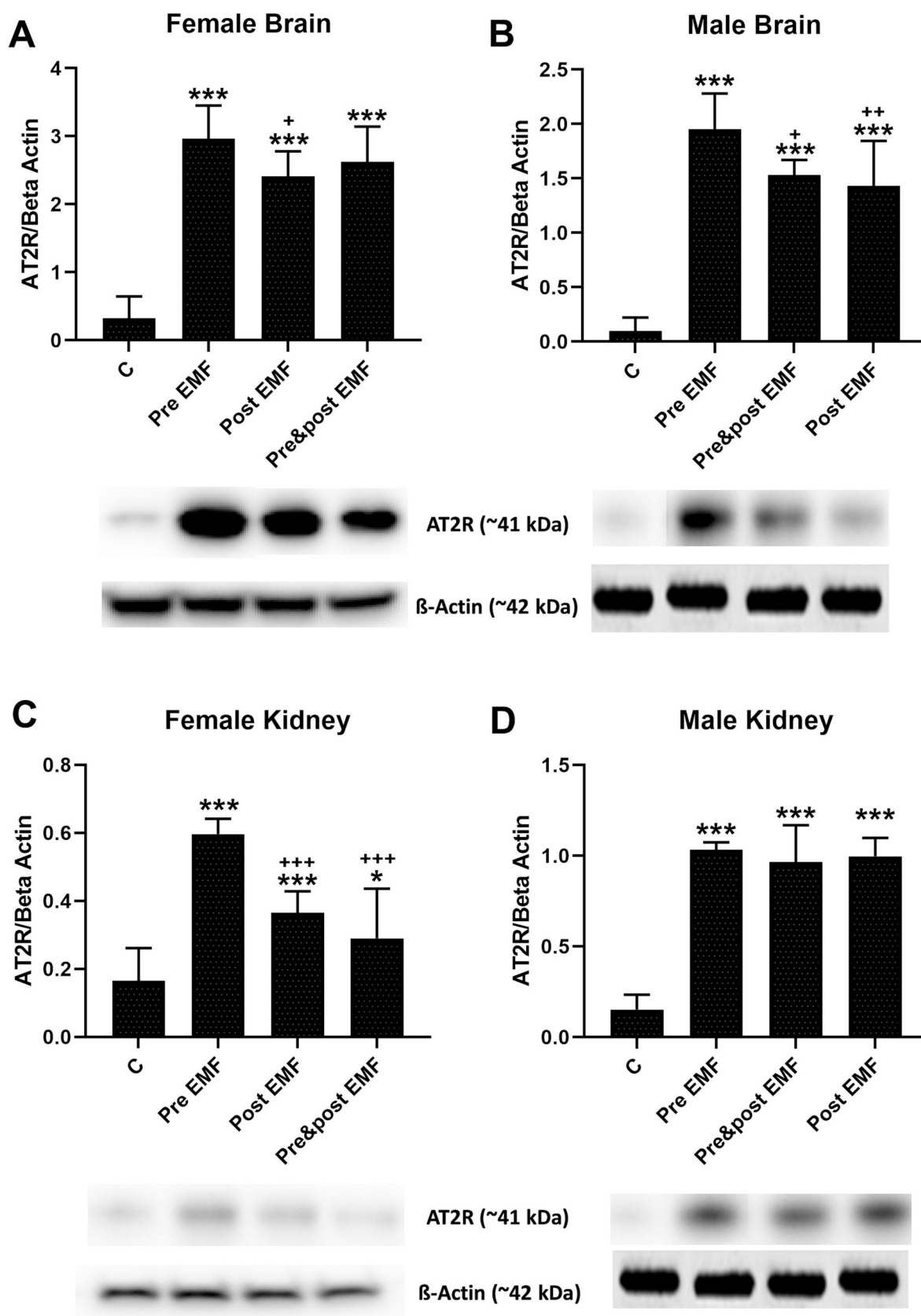
Fig. 6. Western blotting assay results of AT2R for female brain tissue (n = 9) (A), male brain tissue (n = 9) (B), female kidney tissue (n = 9) (C) and male kidney tissue (n = 9) (D). AT2R; Angiotensin II Type 2 Receptor. Data were presented as mean \pm SD. ***P < 0.001 statistical significance compared to C group. +p < 0.05, ++p < 0.01, +++p < 0.001 compared to the Pre EMF group.
