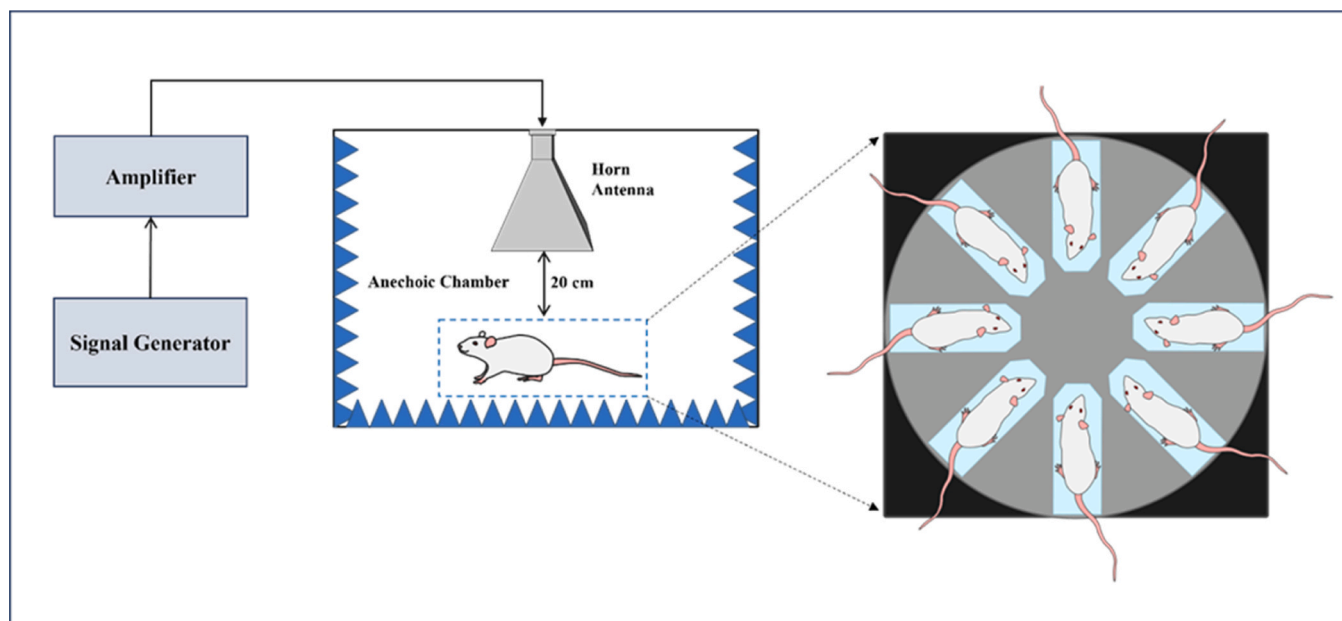
Fig. 2. Schematic representation of the exposure setup.
