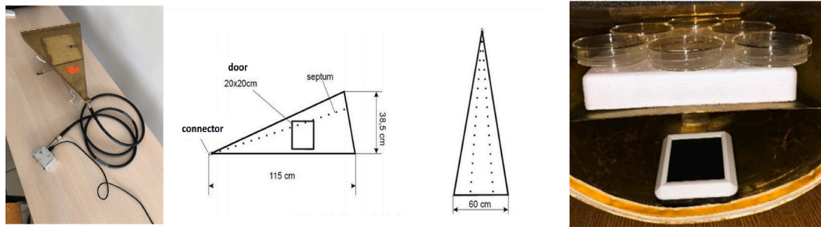
Fig. 1. The gigahertz transverse electromagnetic cell (GTEM) and petri dishes inside a GTEM with a digital thermometer.
