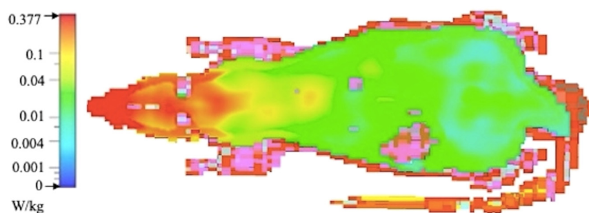
FIGURE 1 Specific absorption rate simulation results at 3500 MHz for 1 g average frontal plane.
