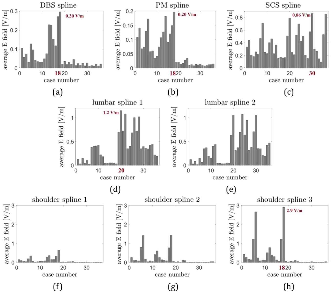
FIGURE 10 | Histograms showing the average tangential E-fields along selected splines exposed to 450 MHz source; the case numbers refer to the positions on Ella's back (see Figure 4(d)), starting at case1 for the top left to case 18 at the bottom right for the source positioned at a distance of 2 mm, and cases 19–36 for the source at 50 mm distance; case numbers corresponding to the highest induced voltages for each spline type are labeled red: (a) DBS, (b) PM, (c) SCS, (d) L1, (e) L2, (f) S1, (g) S2, (h) S3.
