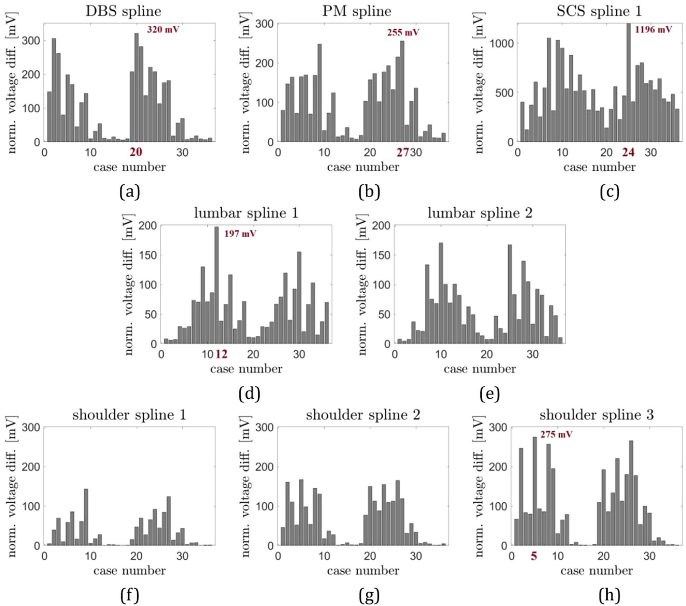
FIGURE 6 | Induced voltage histograms of selected splines exposed to the 85 kHz source; the case numbers refer to the positions on Ella's back (see Figure 4(d)), starting at case1 for the top left to case 18 at the bottom right for the source positioned at a distance of 2 mm, and cases 19–36 for the source at 50 mm distance; case numbers corresponding to the highest induced voltages for each spline type are labeled red: (a) DBS, (b) PM, (c) SCS, (d) L1, (e) L2, (f) S1, (g) S2, and (h) S3.
