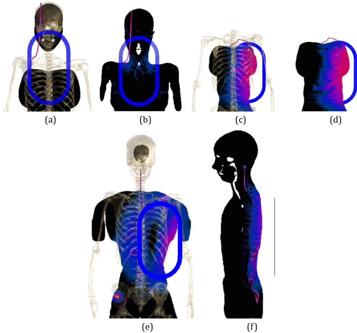
FIGURE 8 | Cross-sectional slices of the maximum field distributions of active implants exposed to the 85 kHz source: (a) xy -slice of the DBS IPG end, (b) xy -slice of the DBS electrode end, (c) xy -slice of the PM IPG end, (d) xy -slice of the PM electrode end, (e) xy -slice of the SCS IPG end, and (f) xz -slice of the SCS electrode end.
