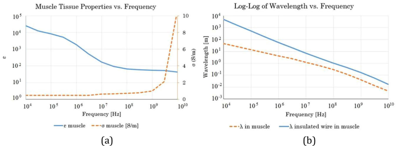
FIGURE 2 | (a) Muscle tissue dielectric properties and (b) wavelength in muscle and King wavelength of an insulated antenna as a function of frequency.
