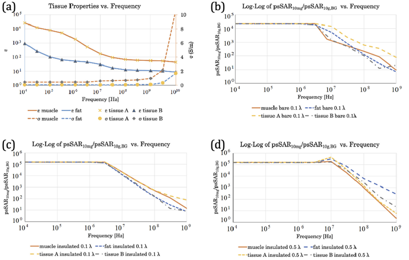
FIGURE 5 | Ratio of the enhanced \text{psSAR}_{10\text{mg}} of simplified implants over background \text{psSAR}_{10\text{g}} as a function of frequency across the range 10^4 – 10^9 Hz in four tissues: muscle (orange), fat (blue), tissue A (yellow), and tissue B (gray); (a) dielectric properties of muscle and fat tissues \epsilon_r (solid line) and \sigma (dashed line), with data for tissues A and B superimposed as markers; (b) enhancement of ratio of the bare implant of length 0.1\lambda ; (c) enhancement ratio of the insulated implant of length 0.1\lambda ; and (d) enhancement ratio of the insulated implant of length 0.5\lambda .
