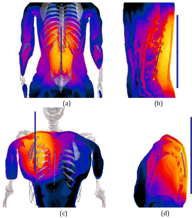
FIGURE 13 | Cross-sectional slices of the maximum field distributions of passive implants exposed to the 450 MHz source: (a) xy -slice of L1, (b) xz -slice of L1, (c) xy -slice of S3, and (d) xz -slice of S3.
