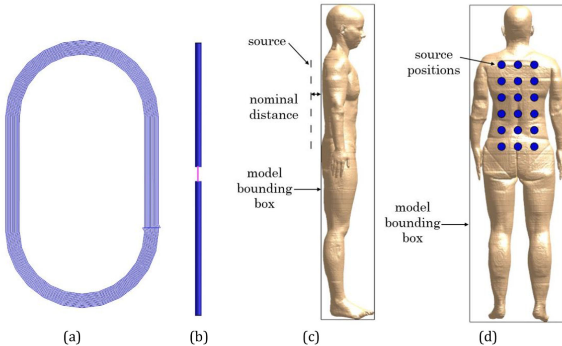
FIGURE 4 | Safety simulation performed with the human anatomical ViP model Ella V3.0: (a) 85 kHz coil source, (b) 450 MHz dipole source (dimensions not to scale), (c) side view, and (d) back view of the source positions and bounding box in proximity to Ella V3.0. were extracted. At 85 kHz, the induced E-field along the splines was extracted and integrated over the implant spline length to determine the voltage difference between the two endpoints (Liorni et al. 2018). At 450 MHz, the average of the tangential E-fields, which is a good metric for the deposited power (ISO 2022), was computed. A summary of the spline lengths as a function of \lambda is given in Table 2.
