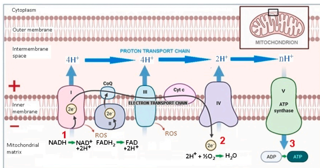
Fig. 1. Electron and proton currents are traced in black and blue, respectively, within the OXPHOS chain. Molecular Complexes are labeled with black Roman numerals (I to V). The diagram is about 200 nm wide. Plus and minus signs in red indicate static polarization of the inner mitochondrial membrane.
