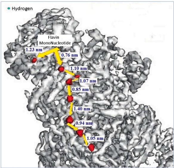
Fig. 2. Electron jumps in Complex I [59].
