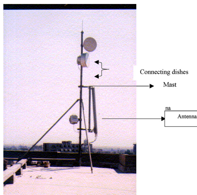
Fig. 2. The antenna of a mobile phone base station upon the building.
