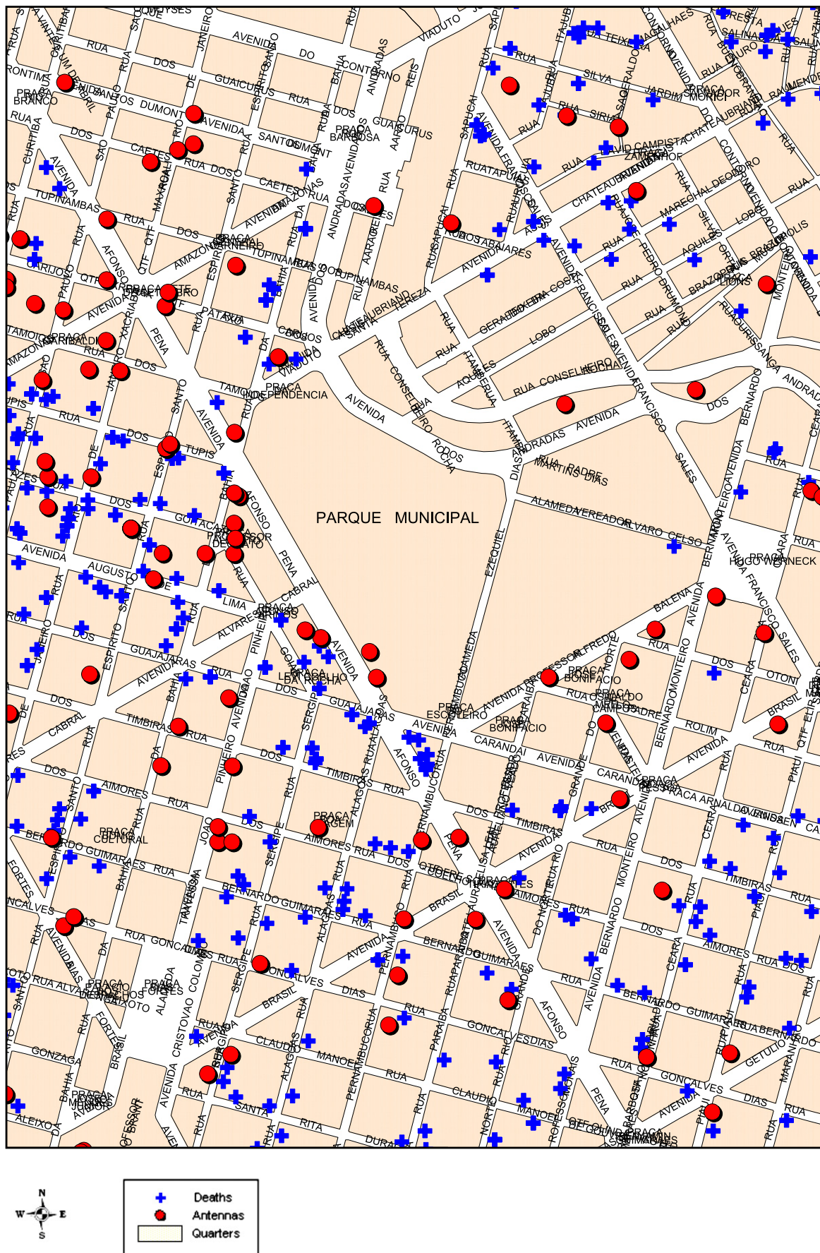
Fig. 10. Sample of geocoded deaths and BS locations in downtown Belo Horizonte City located in Central-Southern region.
