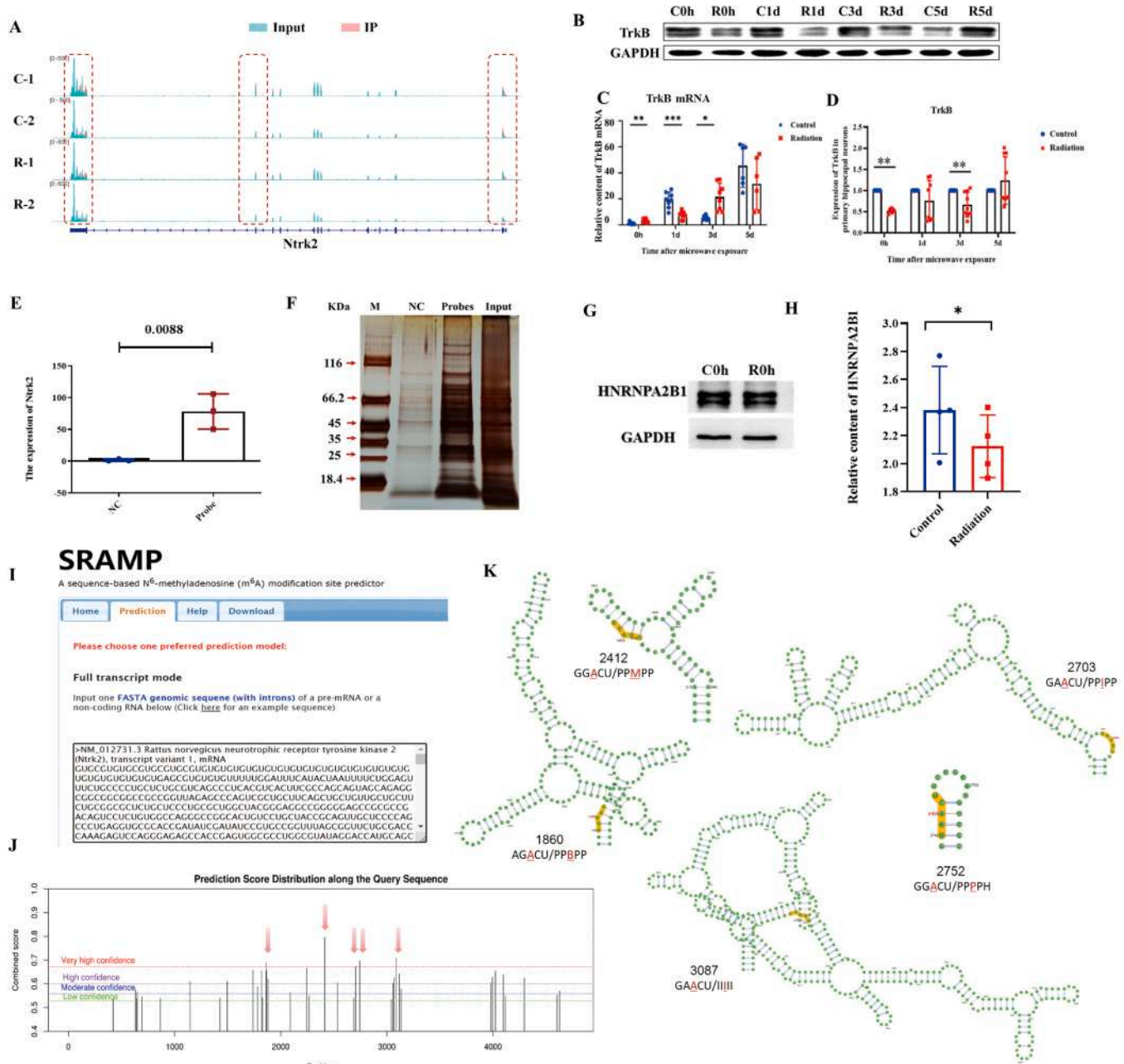
Fig. 7. HNRNPA2B1 down-regulates BDNF expression through feed forward regulation via m^6A -dependent destabilization of TrkB mRNA after microwave radiation. A: m^6A signal in exposure group were decreased at specific positions of TrkB (C-1 and C-2 represent two biological replicates of the sham radiation group; R-1 and R-2 represent two biological replicates of the radiation group, m^6A modification sites with differential expression are indicated by red dashed circles). B: Western blot analysis of TrkB protein expression under the influence of microwave radiation. C: Impact of microwave radiation on TrkB mRNA expression ( n = 6 , the experiment was performed in quadruplicate for each sample, *, p < 0.05 ; **, p < 0.01 ). D: Quantitative analysis of TrkB protein expression by Western blot ( n = 5 , the experiment was conducted 6 times for each sample, *, p < 0.05 ; **, p < 0.01 ). E: q-PCR quantification of TrkB content in TrkB RNA pull-down assay products. F: Silver staining of TrkB RNA pull-down assay. G–H: Effects of microwave radiation on HNRNPA2B1 protein expression-Western blot ( n = 3 , for each sample, the experiment was conducted 4 times, *, p < 0.05 ; **, p < 0.01 ). I–J: Prediction results of TrkB/NTRK2 mRNA in SRAMP website show the potential site of m^6A modification. The red arrow points sites with very high confidence. K: The secondary structure of potential site of m^6A modification on TrkB/NTRK2 mRNA predicted in SRAMP website.
