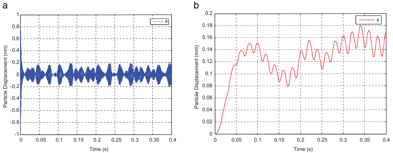
FIG. 7. AC-DC magnetic fields and induced electric field: Here x(0) , y(0) , and z(0) are initial positions and x'(0) , y'(0) , and z'(0) are initial velocities in x , y , and z directions. (a) Bound ion's displacement with time. x(0) = y(0) = z(0) = 10^{-9} m, \omega_0 = 240.75 rad/s, \omega_3 = 10^6 rad/s, \kappa = 1,000 s ^{-1} , and \theta = \pi/4 . The bound ion oscillates and it is not free to displace. (b) Free ion's displacement with time. x(0) = y(0) = z(0) = 10^{-9} m, \omega_0 = 240.75 rad/s, \omega_3 = 1 rad/s, \kappa = 1,000 s ^{-1} , and \theta = \pi/4 .
