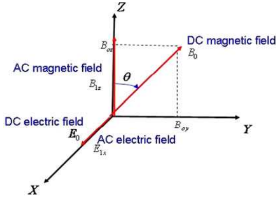
FIG. 2. Coordinate system: DC magnetic field B_0 , AC electric field E , and AC magnetic field B_{1z} . Here, DC magnetic field B_0 is in the vertical y - z plane, a uniform AC electric field E is in x direction perpendicular to the y - z plane, and AC magnetic field B_{1z} is in z direction perpendicular to the x - y plane.
