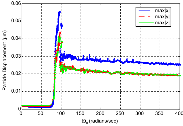
FIG. 3. DC magnetic field: The particle's displacement with DC magnetic field's strength. x(0)=y(0)=z(0)=10^{-9} m, x'(0)=y'(0)=z'(0)=10^{-8} m/s, \omega_3=1 rad/s, \kappa=10 s ^{-1} , and \theta=\pi/4 . Here x(0) , y(0) , and z(0) are initial positions and x'(0) , y'(0) , and z'(0) are initial velocities in x , y and z directions. A resonance occurs at \omega_0=90 rad/s where DC magnetic field strength is 18.7 \mu\text{T} .
