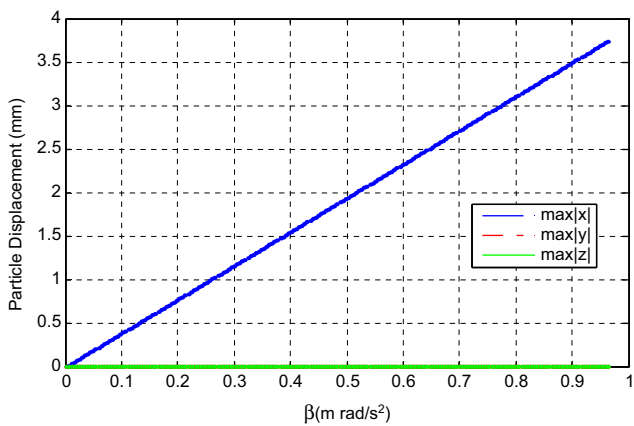
FIG. 4. DC electric field: The particle's displacement with DC electric field's strength. Here, \beta_{ox}=\psi q E_{ox}/m , where E_{ox} is the DC electric field's strength. x(0)=y(0)=z(0)=10^{-9} m, x'(0)=y'(0)=z'(0)=10^{-8} m/s, \omega_3=1 rad/s and \kappa=100 s ^{-1} . Here x(0) , y(0) , and z(0) are initial positions and x'(0) , y'(0) , and z'(0) are initial velocities in x , y , and z directions. The electric field strength ranges from 1 to 20 nV/m. The displacement in x direction linearly increases with increasing electric field intensity, whereas in y and z directions it remains constant across the range of electric field intensity and is lower than the displacement in x direction. The displacement in y and z directions overlaps.
