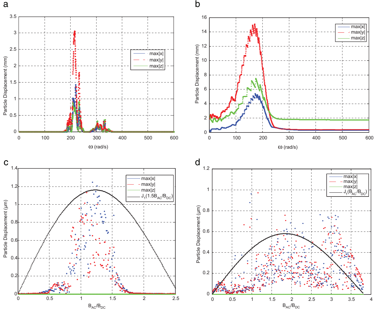
FIG. 6. AC-DC magnetic fields and induced electric field: Here x(0) , y(0) , and z(0) are initial positions and x'(0) , y'(0) , and z'(0) are initial velocities in x , y , and z directions. (a) The particle's displacement with circular frequency of AC magnetic field x(0) = y(0) = z(0) = 10^{-9} m, \omega_1 = 261.68 rad/s, \omega_0 = 240.75 rad/s, \omega_3 = 1 rad/s, \kappa = 10 s ^{-1} , and \theta = \pi/4 . Resonances occur at non-cyclotron frequencies and in the absence of noise. (b) The particle's displacement with circular frequency of AC magnetic field. x(0) = y(0) = z(0) = 10^{-9} m, \omega_1 = 261.68 rad/s, \omega_0 = 240.75 rad/s, \omega_3 = 1 rad/s, \kappa = 100 s ^{-1} , and \theta = \pi/2 . Resonances occur at non-cyclotron frequencies and in the presence of noise. (c) The particle's displacement with B_{AC}/B_{DC} . x(0) = y(0) = z(0) = 10^{-9} m, \omega = \omega_0 = 240.75 rad/s, \omega_3 = 1 rad/s, \kappa = 100 s ^{-1} , and \theta = 0 . Here, the effect of noise is neglected. The particle follows the Bessel function J_1(1.5B_{AC}/B_{DC}) when magnetic fields are parallel and induced electric field is considered. This does not predict the Ion Parametric Resonance model. (d) The particle's displacement with B_{AC}/B_{DC} . x(0) = y(0) = z(0) = 10^{-9} m, \omega = \omega_0 = 240.75 rad/s, \omega_3 = 1 rad/s, \kappa = 10 s ^{-1} , and \theta = 0 . Here, the effect of induced electric field and noise is neglected. The particle follows the Bessel function J_1(B_{AC}/B_{DC}) when magnetic fields are parallel. This predicts the Ion Parametric Resonance model.
