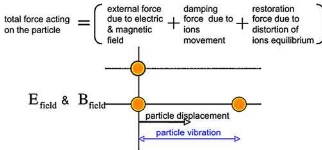
FIG. 1. Total force acting on the charged particle due to electric and magnetic fields.
