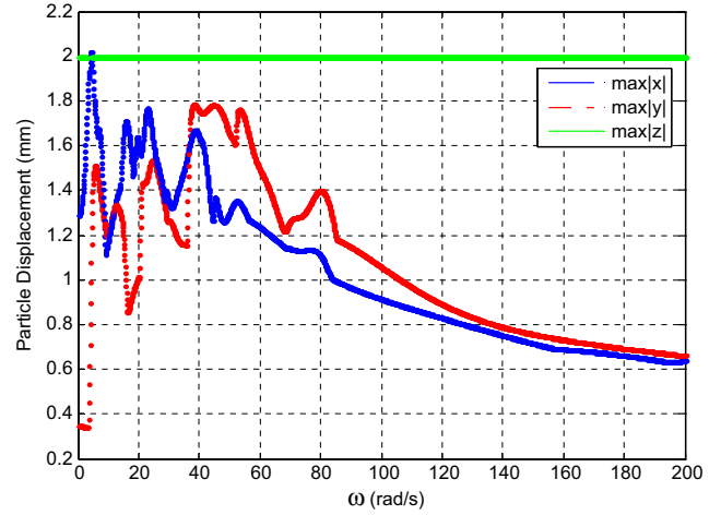
FIG. 5. AC magnetic field and induced electric field: The particle's displacement with circular frequency of AC magnetic field. x(0)=y(0)=z(0)=10^{-9} m, \omega_1=261.68 rad/s, \omega_3=1 rad/s and \kappa=100 s ^{-1} . Here x(0) , y(0) , and z(0) are initial positions and x'(0) , y'(0) , and z'(0) are initial velocities in x , y , and z directions. Several resonances occur even in the absence of a DC magnetic field in x and y directions, whereas in z direction, displacement does not vary with the angular frequency.
