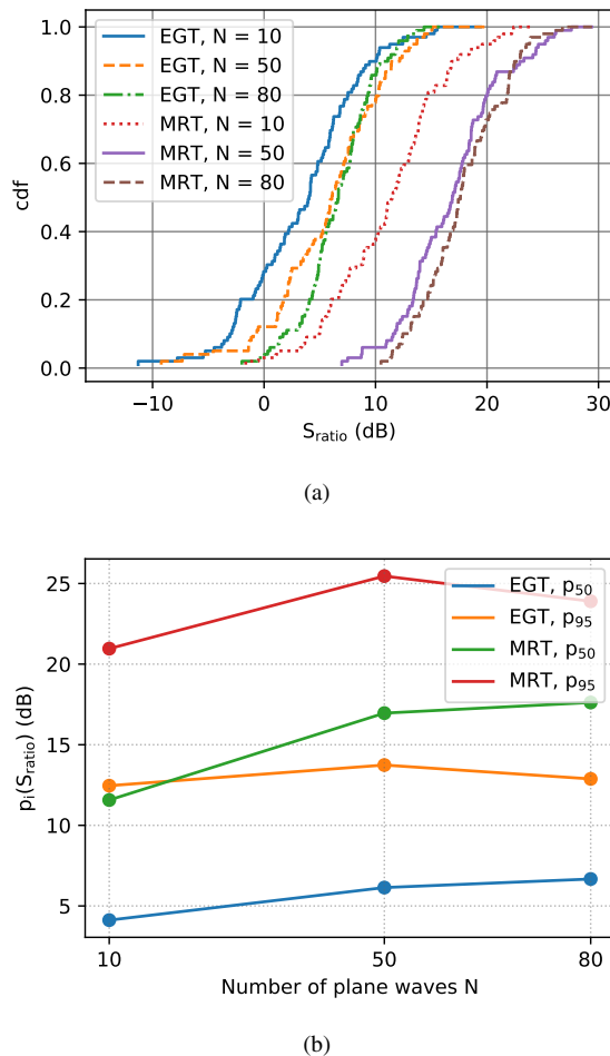
FIGURE 4. (a) Cumulative distribution function (cdf) of S_{ratio} for a different number of plane wave sources N . (b) The 50th and 95th percentiles of S_{ratio} as a function of number of incident plane waves.
