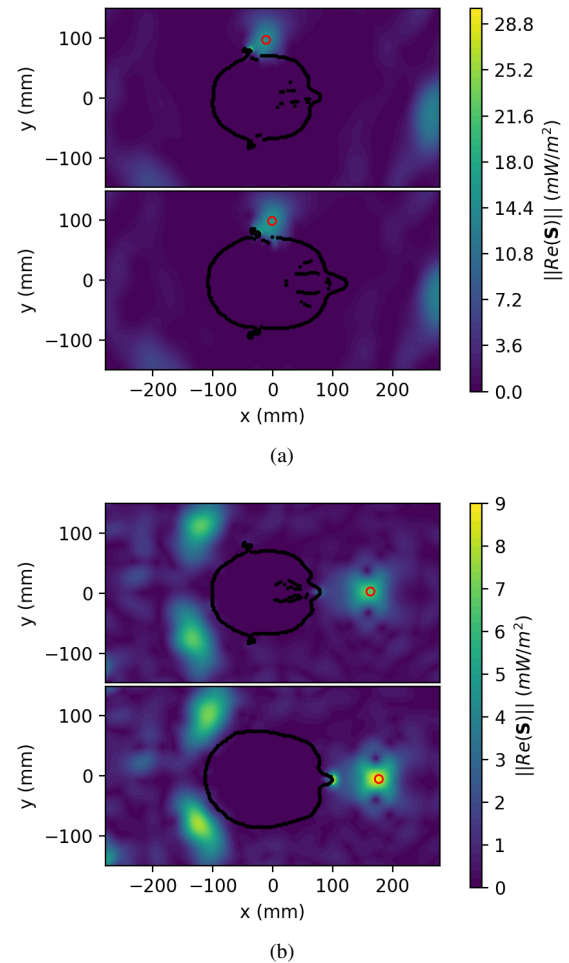
FIGURE 5. The power density focused at the UE (red circle) located (a) next to the ear and (b) in front of the eyes in the xy -plane ( z = z_{focus} ) for the Ella (top) and Duke (bottom) phantom using MRT precoding. The precoding weights are normalized according to (2).
