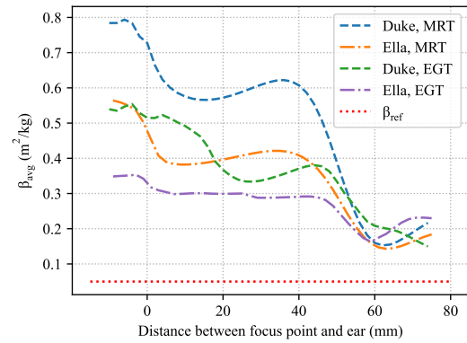
FIGURE 8. psSAR 10g (basic restriction) normalized to the average incident power density (reference level) over the computational domain, i.e., 560 mm × 300 mm × 250 mm ( \beta_{\text{avg}} ) as a function of distance. The UE is located next to the ear. The red dotted line ( \beta = 0.05 \text{ m}^2/\text{kg} ) indicates the reference value obtained with the ICNIRP guidelines for the general public.
