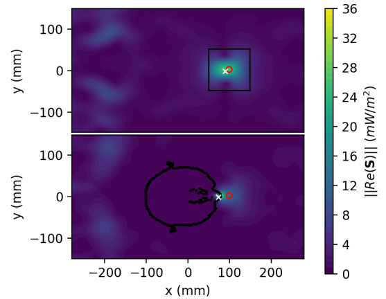
FIGURE 3. Illustration of the different definitions of S_{\text{inc}} (reference level). The power density focused at the UE located in front of the eyes in the xy -plane ( z = z_{\text{focus}} ) for the Ella phantom using MRT precoding. The precoding weights are normalized according to (2). The power density without (top, normalization 2) and with (bottom) phantom is shown. White cross: maximum power density (top, normalization 1). Red circle: focus point (bottom, normalization 3). Black square: averaging volume V_{\text{avg}} = 100 \text{ mm} \times 100 \text{ mm} \times 100 \text{ mm} (top, normalization 4).
