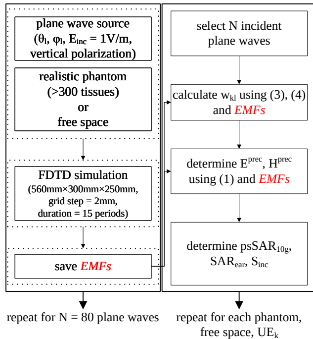
FIGURE 1. Scheme of the chosen methodology consisting of plane wave simulations and precoding and how these intersect.
