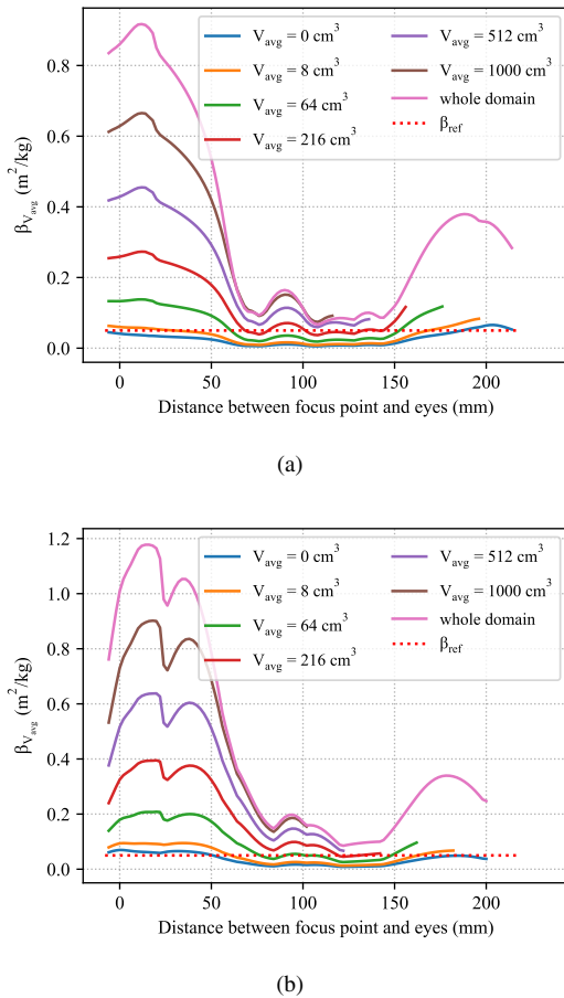
FIGURE 11. psSAR 10g (basic restriction) normalized to S_{inc, V_{avg}} (reference level) leading to \beta_{V_{avg}} as a function of distance for the (a) Ella and (b) Duke phantoms using MRT. The UE is located in front of the eyes. The red dotted line ( \beta = 0.05 m^2/kg ) indicates the reference value obtained with the ICNIRP guidelines for the general public.
