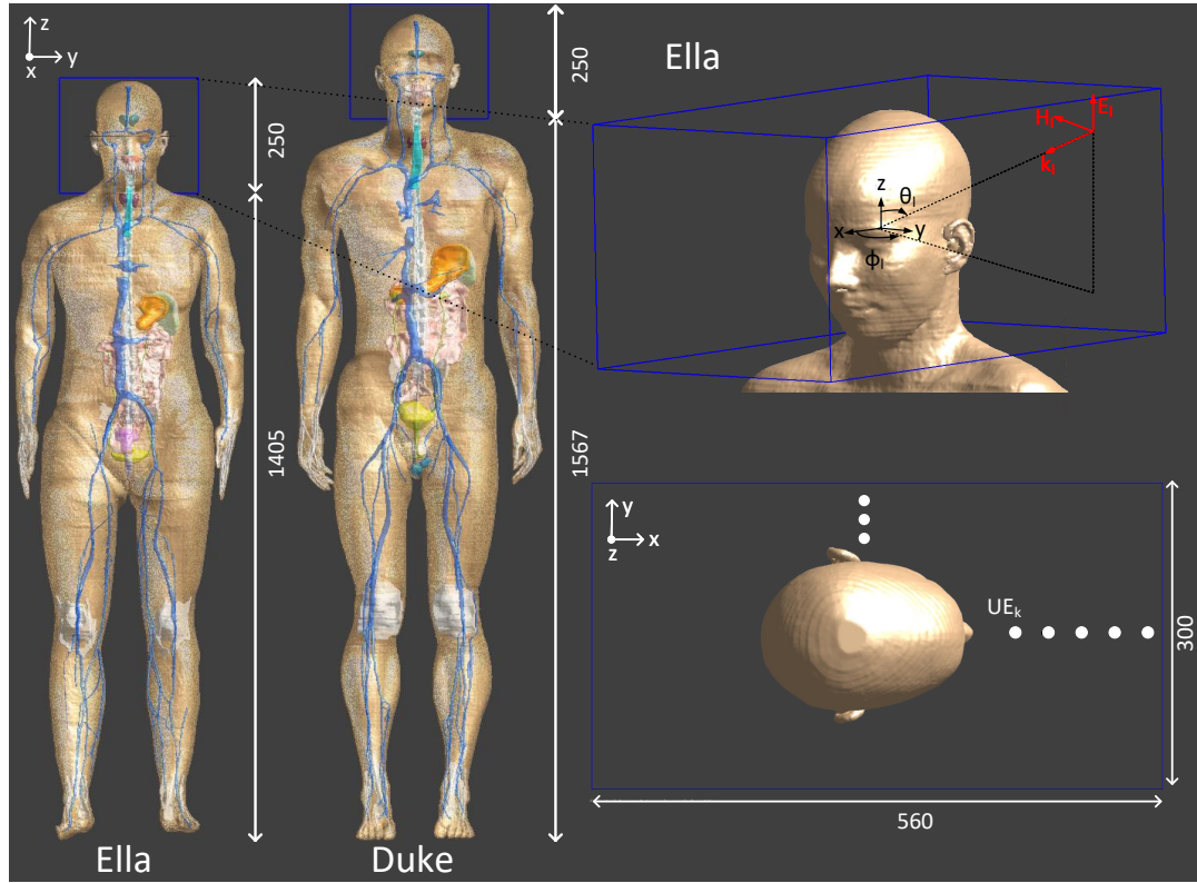
FIGURE 2. Simulation setup. The FDTD domain (560 mm × 300 mm × 250 mm) is indicated by the blue box. Left: whole-body phantoms. Top right: The Ella phantom with incident plane wave l in red. Bottom right: Top view of the Ella phantom with the possible locations of UE k , i.e., next to ear and in front of eyes and nose, shown by the white dots. All dimensions are given in mm.
