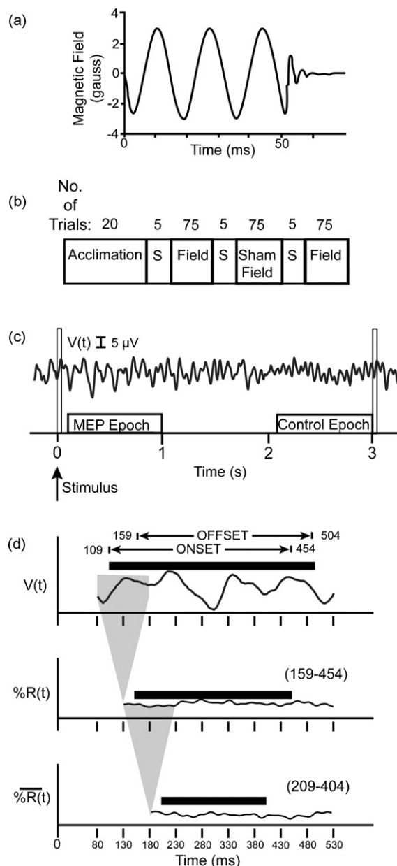
Fig. 1. Experimental design and procedure. (a) Applied magnetic stimulus (60 Hz shown). (b) Organization of trials in an experimental session. S, sound stimulus. (c) An EEG trial showing the locations of the epoch containing the magnetosensory evoked potential (MEP) and the corresponding control epoch. (d) Convention for synchronizing the graphical representation of related time series. The bar depicts the expected latency range for the MEP (superposition of the onset and offset MEPs). The stippled regions indicate the relation between the deterministic behavior in one time series and where that behavior was represented after analysis.
