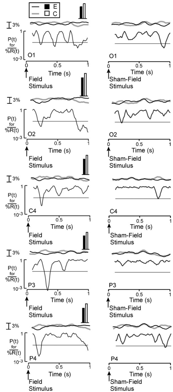
Fig. 4. Results obtained after filtering the EEG signals from subject S7 exposed to a 60-Hz stimulus using \overline{\%R(t)} . The EEGs had been digitally filtered to remove the 8–10 Hz components. The curves at the top of the panels show the average values of the exposed (E) and control (C) epochs for \overline{\%R(t)} in the exposed (left) and sham-exposed (right) trials ( N \geq 50 trials). P(t) , probability of a difference in means at time t . Bar graphs (drawn to the indicated scale) show the average value of \overline{\%R(t)} over the latency interval for which P(t) < 0.05 (the standard deviations are not resolved at scale shown). MEPs were not detected in the unfiltered EEG (Table 1).
