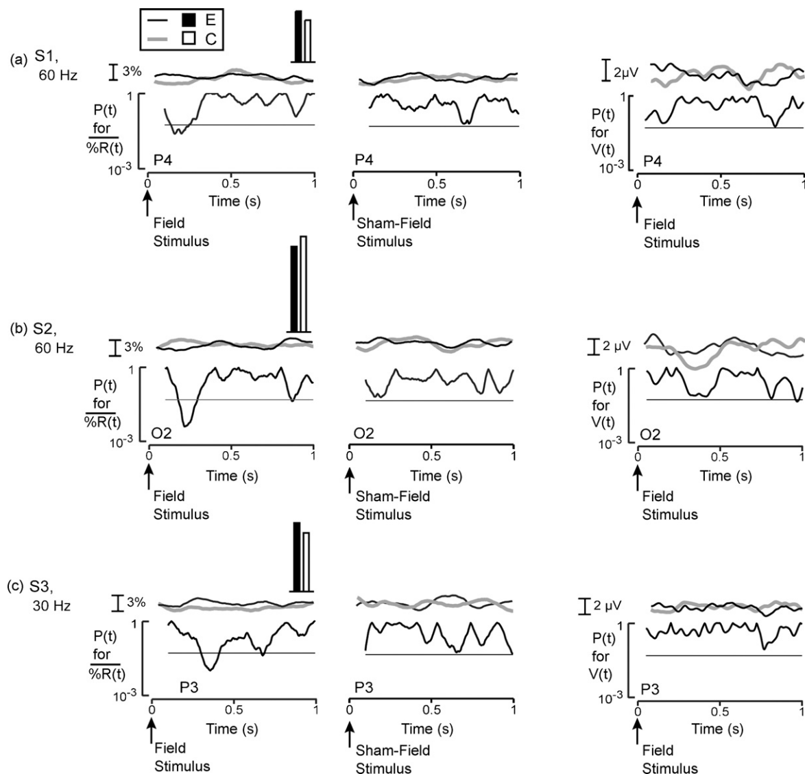
Fig. 2. Magnetosensory evoked potentials detected in three subjects using the recurrence analysis variable \%R(t) . (a, b, c) Subjects S1, S2, S3, respectively. First column, field-stimulus trials; second column, sham-stimulus trials; third column, EEG from which \%R(t) in the field-stimulus trials was computed. The curves at the top of each panel show the average values of the exposed (E) and control (C) epochs for the respective time series ( N \geq 50 trials). P(t) , probability of a difference in means at time t . Bar graphs (drawn to the indicated scale) indicate the average value of \%R over the latency interval for which P(t) < 0.05 (the standard deviations are not resolved at scale shown). The field stimulus was applied for 50 ms.
