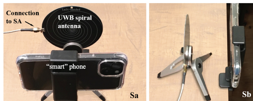
Figure 5. Measurement setup with “smart” phone and RF spiral antenna at 10 cm connected to the SA, as seen from two different angles.
