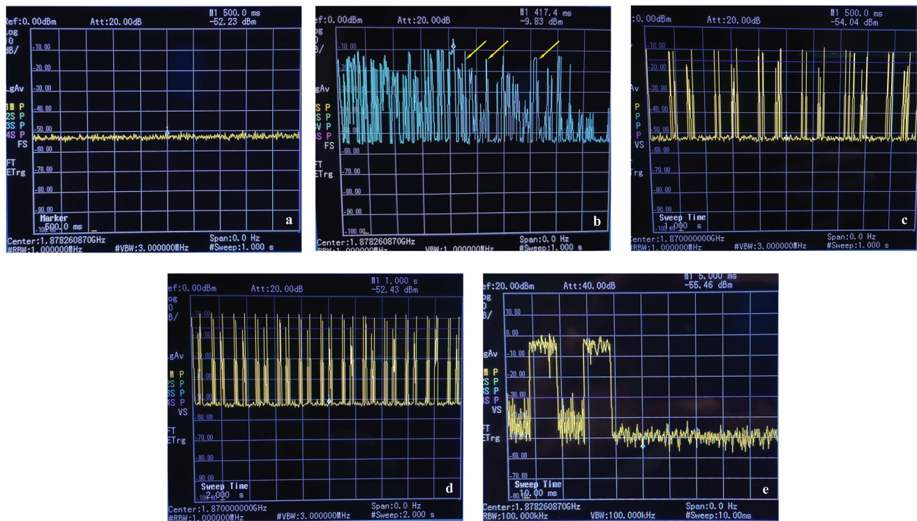
Figure 3. (a): Background (control) recording for NR (5G) with “smart” phone and other RF sources turned off. Center frequency: \sim 1.878 GHz. Sweep time: 1 s. (b): NR (5G) \sim 100 Hz pulses (frames) of (up to) 10 ms duration each (arrows), from the “smart” phone during an active phone call with another phone. Center frequency: \sim 1.878 GHz. Sweep time: 1 s. (c): NR (5G) groups of 2–3 frames, repeated at \sim 13 Hz. Center frequency: \sim 1.87 GHz. Sweep time: 1 s. (d): A similar NR (5G) emission pattern as in Figure 3(c), with groups of 2–3 frames repeated at \sim 13 Hz. Center frequency: \sim 1.87 GHz. Sweep time: 2 s. (e): NR (5G) sub-frames of \sim 1 ms duration each, repeated at \sim 500 Hz. Center frequency: \sim 1.878 GHz. Sweep time: 10 ms.
