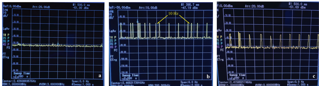
Figure 1. (a) Background (control) recording for Wi-Fi (2.45 GHz) with router and all RF sources turned off. Center frequency: \sim 2.43 GHz. Sweep time: 1 s. (b): \sim 5 – 20 Hz pulses from the Wi-Fi router. Arrows indicate pulses with \sim 10 Hz repetition. Center frequency: \sim 2.46 GHz. Sweep time: 2 s. (c): Pulses with \sim 10 Hz repetition frequency emitted by the Wi-Fi router. Center frequency: \sim 2.42 GHz. Sweep time: 1 s.
