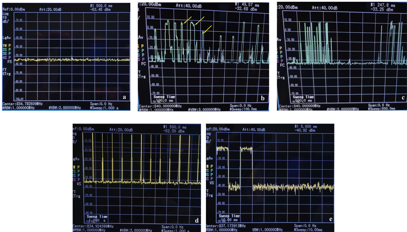
Figure 2. (a): Background (control) recording for LTE (4 G) with “smart” phone and other RF sources turned off. Center frequency: ~835 MHz. Sweep time: 1 s. (b): LTE (4 G) ~100 Hz pulses (“frames”) of ~2–10 ms duration each and variable amplitudes (arrows), emitted by the “smart” phone. Center frequency: 840 MHz. Sweep time: 100 ms. (c): LTE (4 G) pulses (“frames”) of ~5 ms duration each, with ~100 Hz repetition frequency from the “smart” phone, emitted in bursts of ~100 ms duration (“multi-frames”) repeated at a rate of ~3 Hz. Center frequency: 840 MHz. Sweep time: 500 ms. (d): LTE (4 G) pulses, probably for synchronization or reference purposes, repeated at a rate of ~12.5 Hz. Center frequency: ~835 MHz. Sweep time: 1 s. (e): LTE (4 G) sub-frames of ~1 ms duration each, repeated at a rate of ~500 Hz. Center frequency: ~837 MHz. Sweep time: 10 ms.
