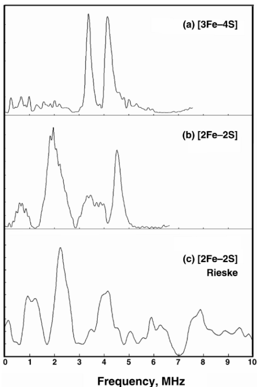
Figure 2. X-band ESEEM spectroscopy illustrates (a) the [3Fe–4S] cluster in fumarate reductase from E. coli ; (b) the [2Fe–2S] ferredoxin from A. platensis ; (c) the Riese protein in bovine heart mitochondria. Adapted from [12].
