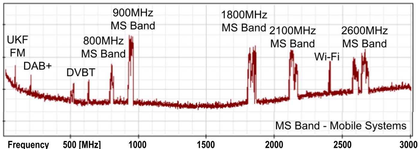
Fig 1. Electromagnetic spectrum used by major radiocommunication systems in Poland.
