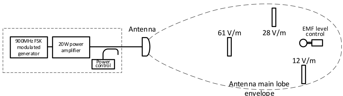
Fig 2. Exposure setup scheme with EMF level control system.
