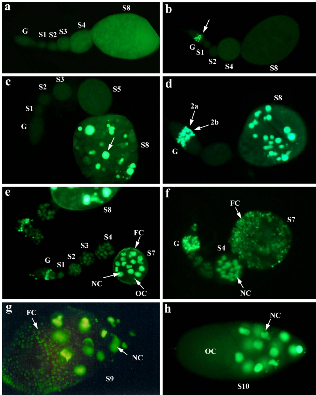
Fig. 1. (a) Typical TUNEL-negative fluorescent picture of an ovariole of a sham-exposed/control female insect, containing egg chambers from germarium up to stage 8. (b) Ovariole of an exposed insect with fragmented DNA only on cells of the germarium 2a/2b region (arrow). (c) Ovariole of an exposed insect with TUNEL-positive signal only at the nurse cells of a stage 8 egg chamber (arrow) and TUNEL-negative at all other stages. (d) Ovariole of an exposed insect with TUNEL-positive signal only at the two checkpoints, regions 2a and 2b of the germarium plus stage 8 egg chamber and TUNEL-negative intermediate stages. (e) Ovarioles of exposed female insects with fragmented DNA at all stages from germarium to stages 7 and 8 and in all kinds of egg chamber cells, (NC: nurse cells, FC: follicle cells, OC: oocyte). (f) Characteristic picture of TUNEL-positive signal in the follicle cells (FC) of a stage-7 egg chamber in an ovariole of an exposed female insect. At the stage-4 egg chamber, cell death appears in the nurse cells (NC). (g) Characteristic picture of induced cell death in the nurse cells (NC) and follicle cells (FC) of a stage-9 egg chamber of an exposed female insect. (h) Stage 10, TUNEL-positive egg chamber of an exposed female insect.
