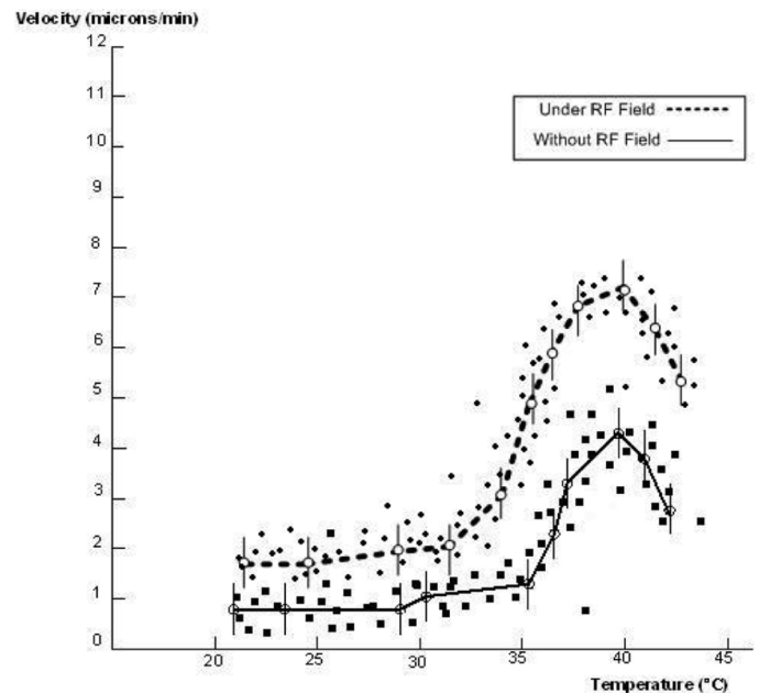
Fig. 3. Cell Velocity as a function of temperature with and without exposure to RF fields at 900 MHz and approximately 0.4 V/m.
