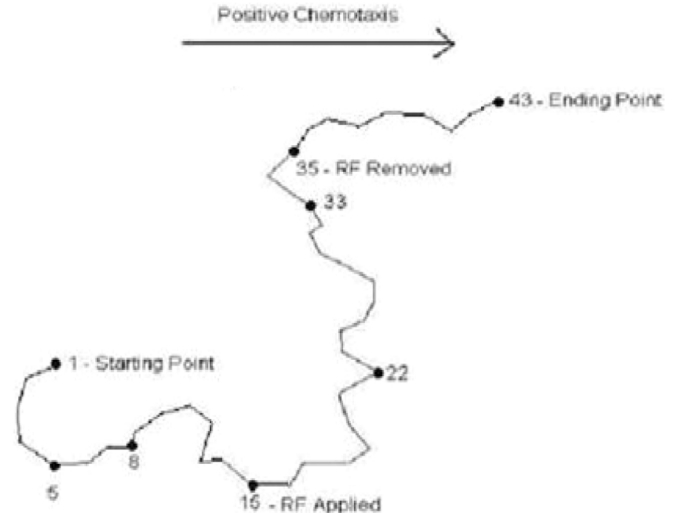
Fig. 2. Typical movement of a neutrophil with RF excitation.
