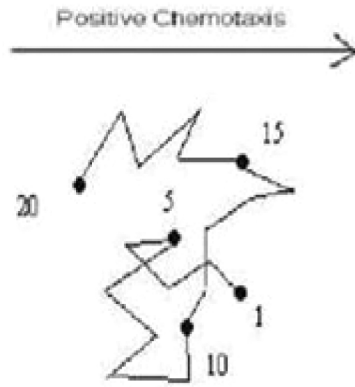
Fig. 1. Random movement of a neutrophil.
